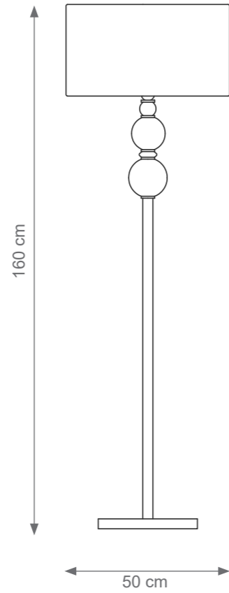
Rita Floor Lamp Code: F807845 Type 1 lights electrification x Max 28W E14 CE Size: cm. 160 h x 50 ø - 12 kg
