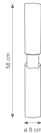
Drum Small Wall Light Code: F807557 Type 1 electrification Led Light Size: cm. 58 h x 8 ø - 1,2 kg
