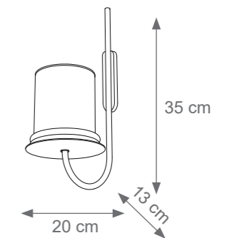
London Applique Code: L807296 Type 1 lights electrification x Max 28W E14 CE Size: cm. 35 h x 20 l x 13 w - 1 kg
