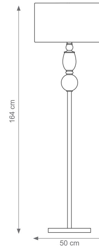
Avaa Floor Lamp Code: F807937 Type 1 lights electrification x Max 28W E14 CE Size: cm. 164 h x 50 ø - 12 kg
